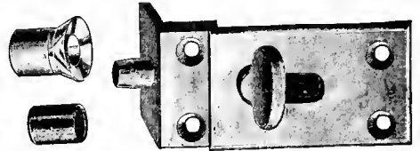
Figs. 4407-4408. BLIND-BOLT BUSHING.
